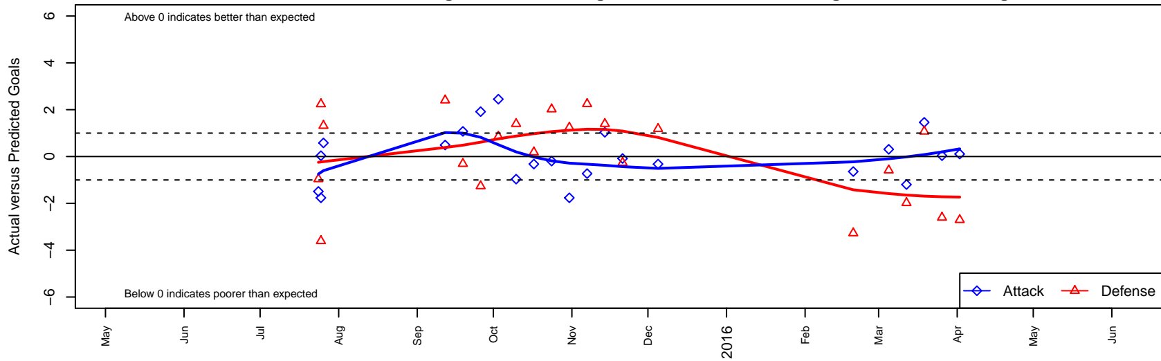
South Whidbey Tsunami B03 Dots are actual minus expected GF (blue circles) and GA (red triangles). Blue line is smoothed change in attack strength. Red is smoothed change in defense strength.
